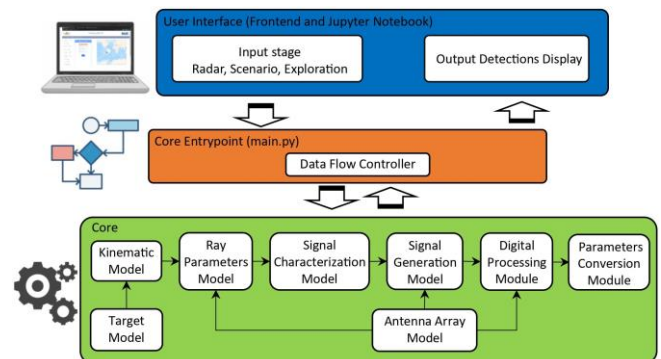
Fig. 4. Implementation scheme of (OTH-SW) Radar Simulation software.
