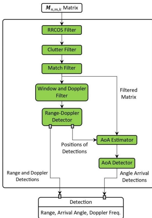
Fig. 16. Digital signal and data processing module.
