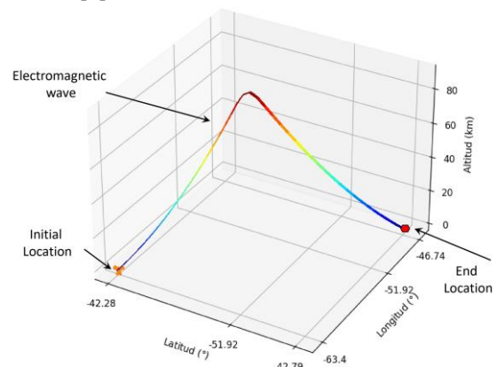
Fig. 13. Example of the path followed by an electromagnetic wave between two points on the Earth's surface. The wave has a carrier
