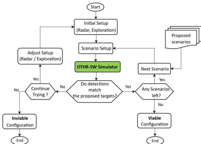
Fig. 2. Evaluation process of a radar configuration against search scenario.
