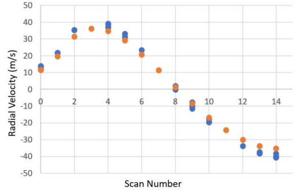
Fig. 21. Detected (in blue) and proposed (in orange) target radial velocities over the 15 scans.
