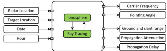
Fig. 12. Ray Parameters Model. Input and output parameters, submodels of Earth's Ionosphere and Ray Tracer.
