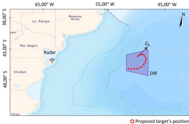
Fig. 19. Representation of the radar system positions, search area, and the target's trajectory.
