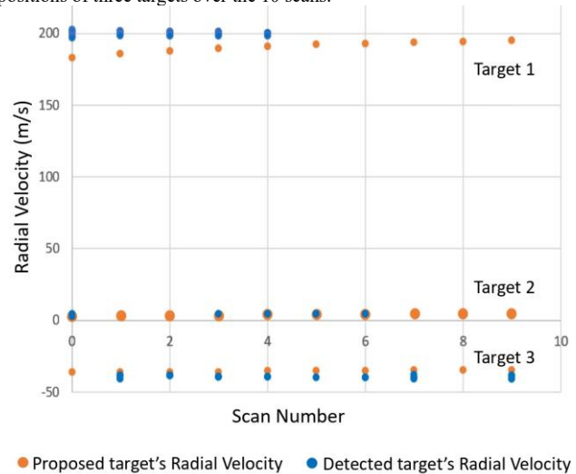
Fig. 25. Detected (in blue) and proposed (in orange) radial velocities of three targets over the 10 scans.
